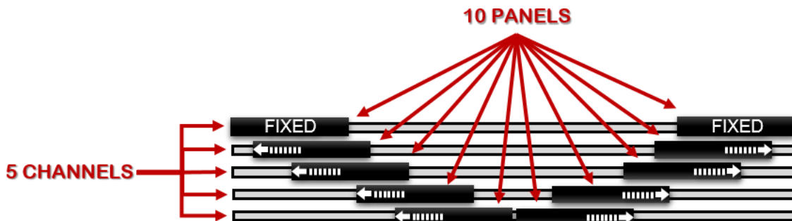
SPLIT DRAW, 5-CHANNEL TRACK, 10 PANELS.
