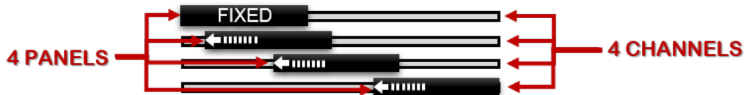
ONE WAY DRAW, 4-CHANNEL TRACK, 4-PANELS
